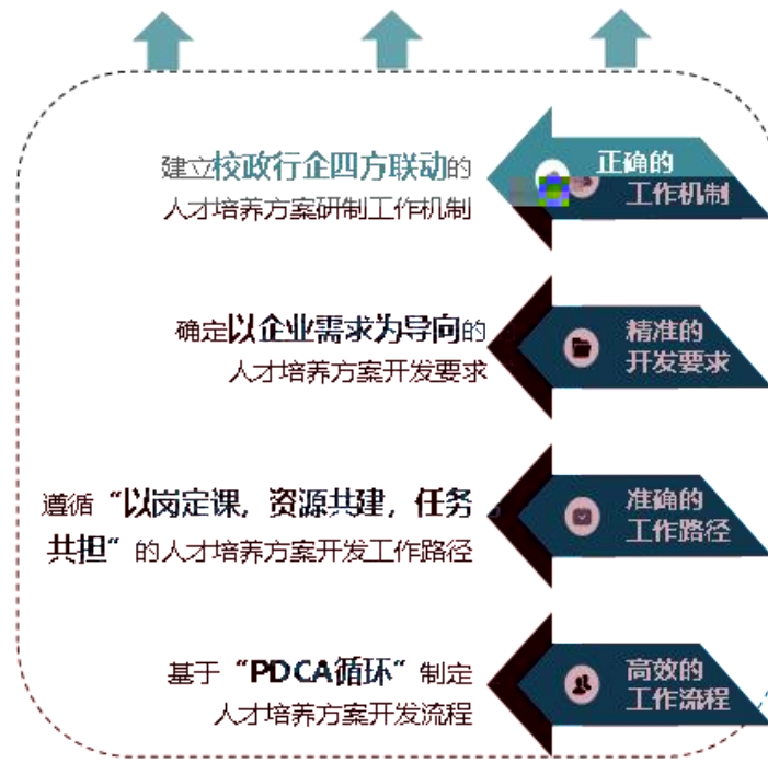
1 PDCA
